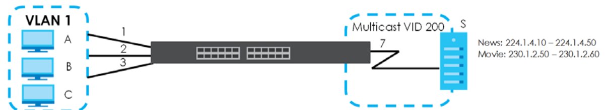
Figure 242 MVR Configuration Example
