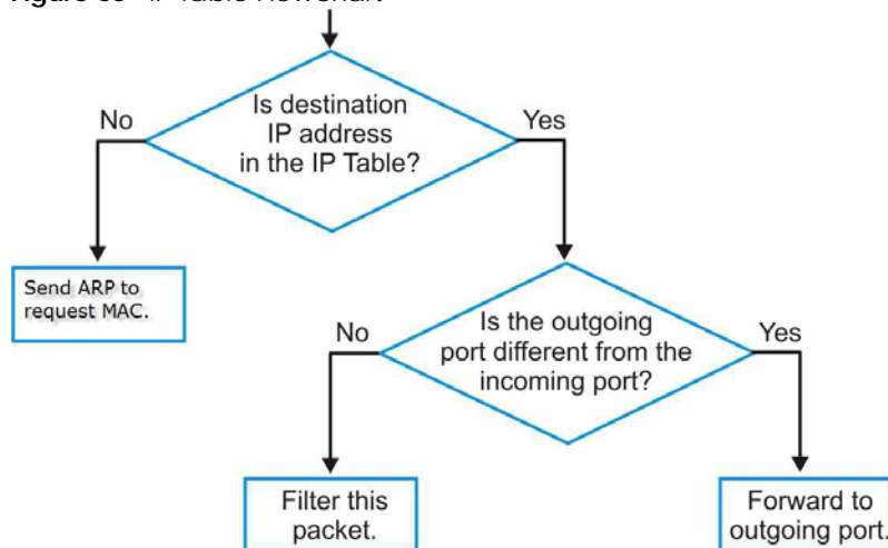
Figure 65 IP Table Flowchart
