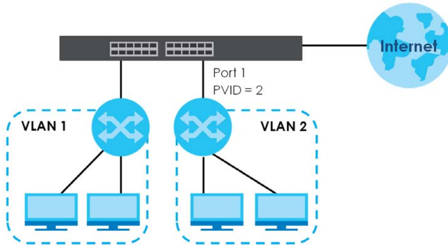
Figure 54 Initial Setup Network Example: Port VID
