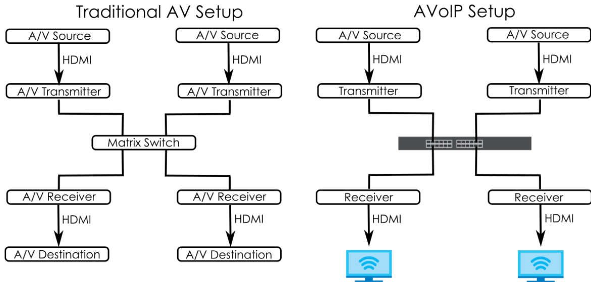
Figure 5 Comparison Between Traditional AV and AVoIP Setups
