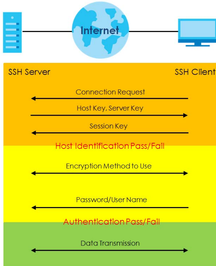
Figure 440 How SSH Works
