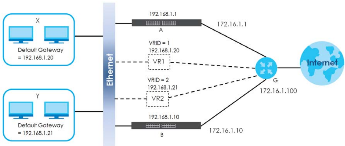
Figure 427 VRRP Configuration Example: Two Virtual Router Network
