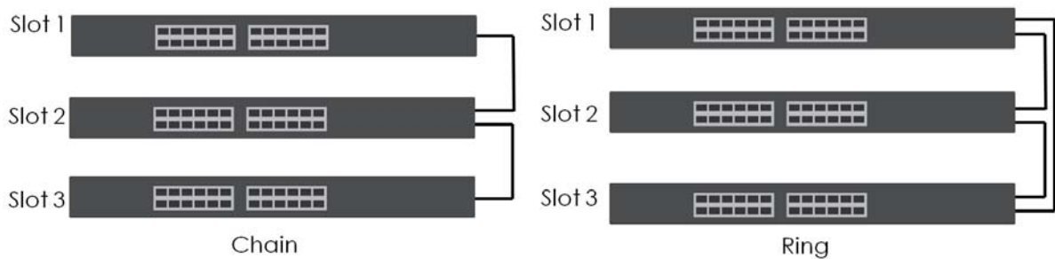
Figure 130 Stacking Topology
