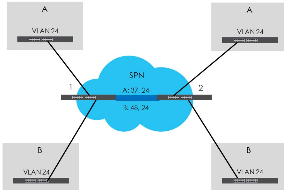
Figure 343 VLAN Stacking Example
