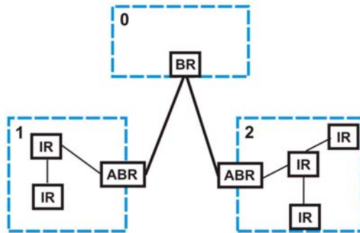
Figure 395 OSPF Network Example
