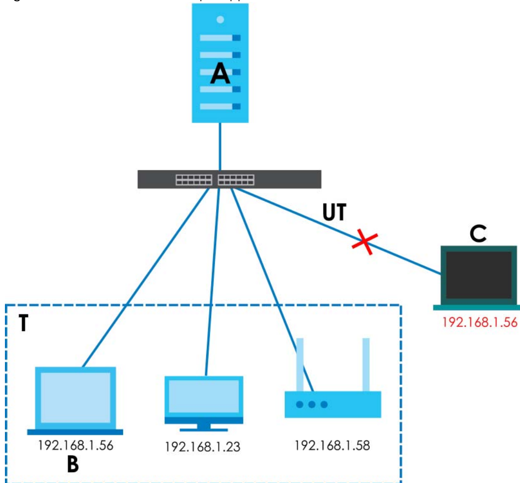
Figure 473 IP Source Guard Example Application
