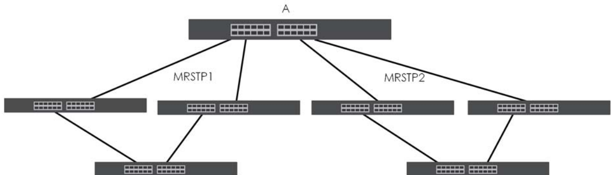
Figure 277 MRSTP Network Example
