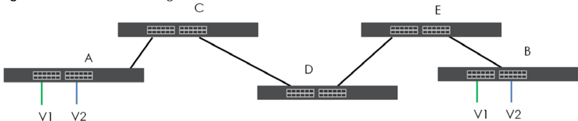
Figure 305 Port VLAN Trunking
