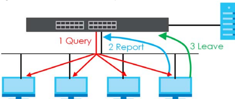
Figure 387 IGMP Version 2 Example
