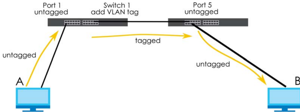
Figure 581 VLAN Forwarding Frame
