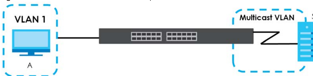
Figure 217 MVR Multicast Television Example
