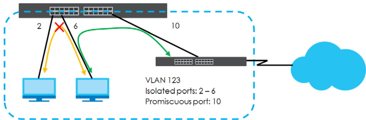
Figure 334 VLAN Isolation Example
