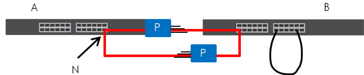
Figure 197 Loop Guard – Probe Packet
