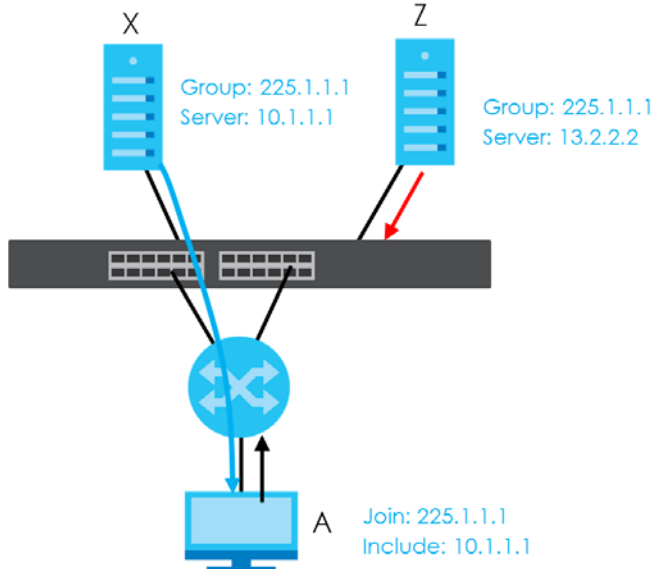
Figure 388 IGMP Version 3 Example
