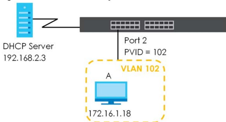
Figure 57 Tutorial: DHCP Relay Scenario
