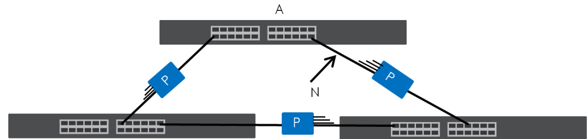
Figure 198 Loop Guard – Network Loop
