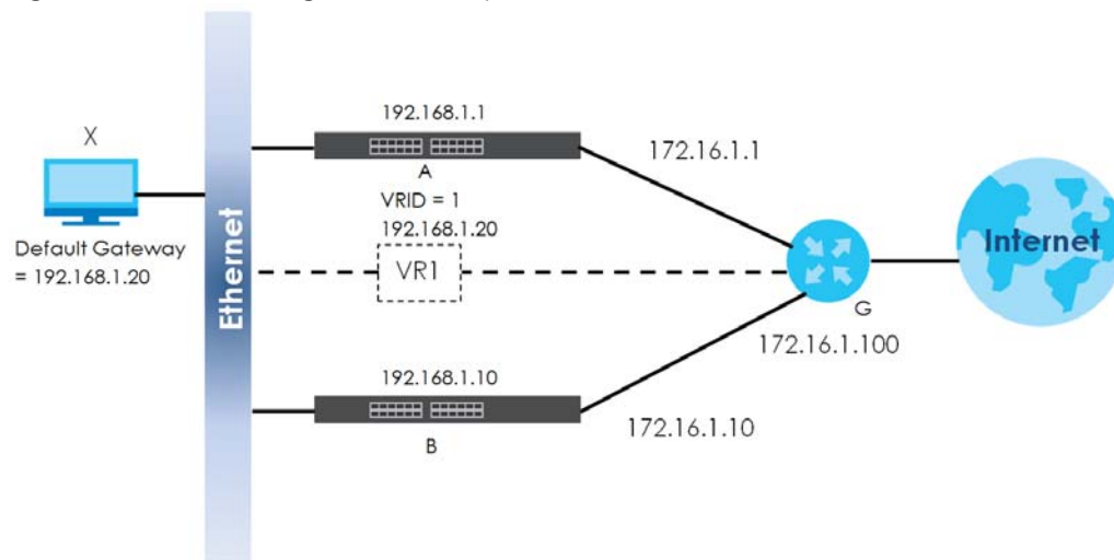
Figure 422 VRRP Configuration Example: One Virtual Router Network
