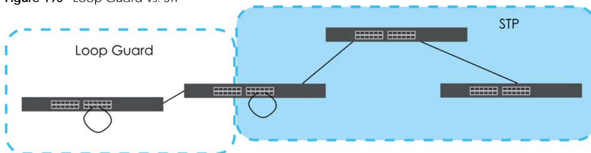
Figure 195 Loop Guard vs. STP
