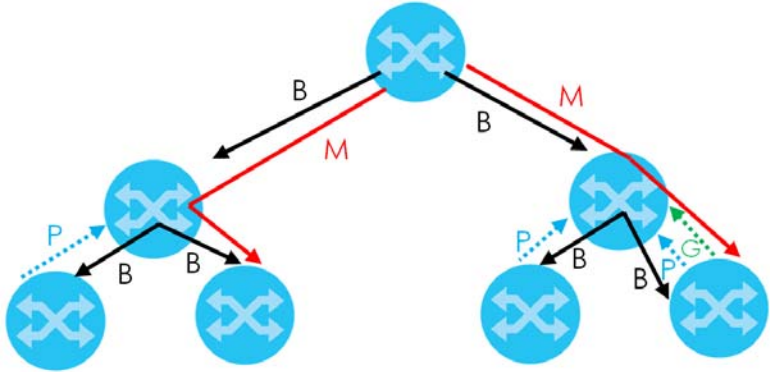
Figure 383 How DVMRP Works
