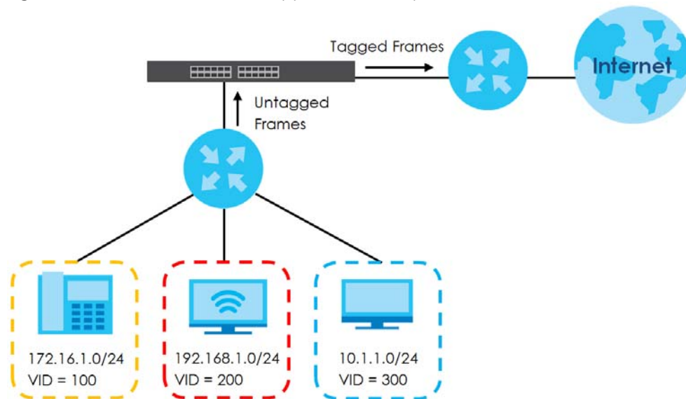
Figure 318 Subnet Based VLAN Application Example
