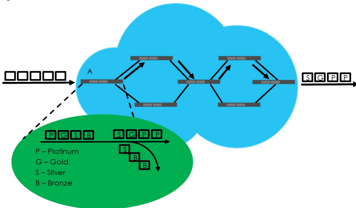
Figure 263 DiffServ Network
