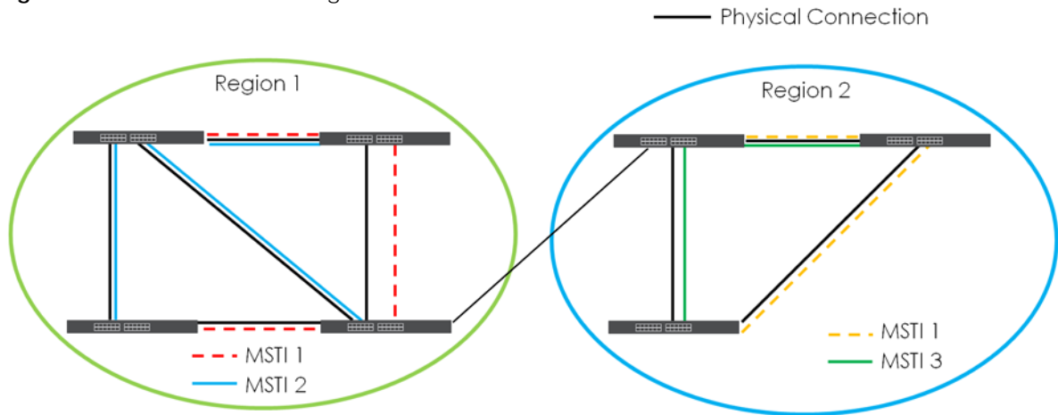
Figure 298 MSTIs in Different Regions
