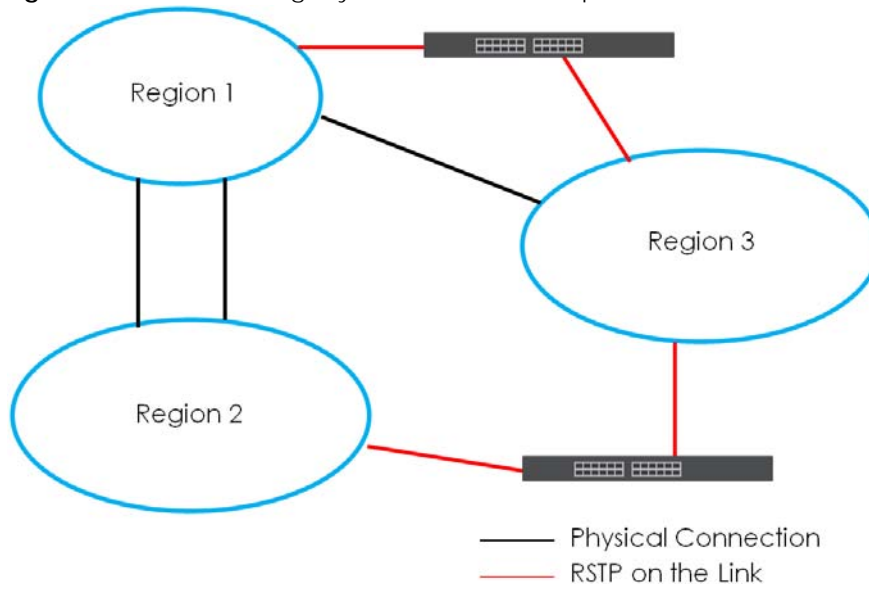
Figure 299 MSTP and Legacy RSTP Network Example
