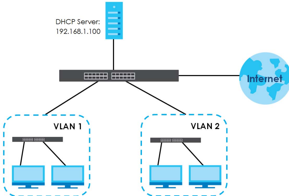
Figure 363 DHCP Smart Relay Network Example
