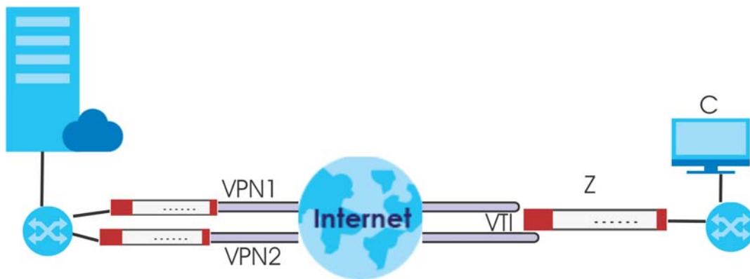
Figure 291 VTI and Trunk for VPN Load Balancing
