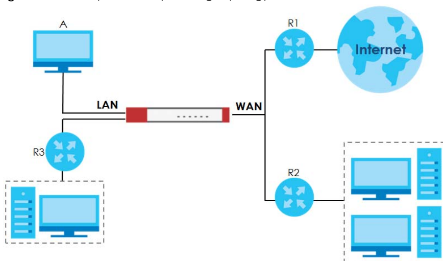
Figure 301 Example of Policy Routing Topology
