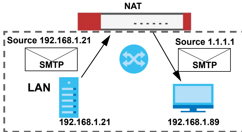
Figure 328 LAN to LAN Return Traffic
