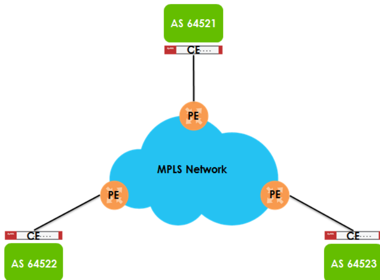
Figure 319 Scenario 1: CE Router - to - MPLS
