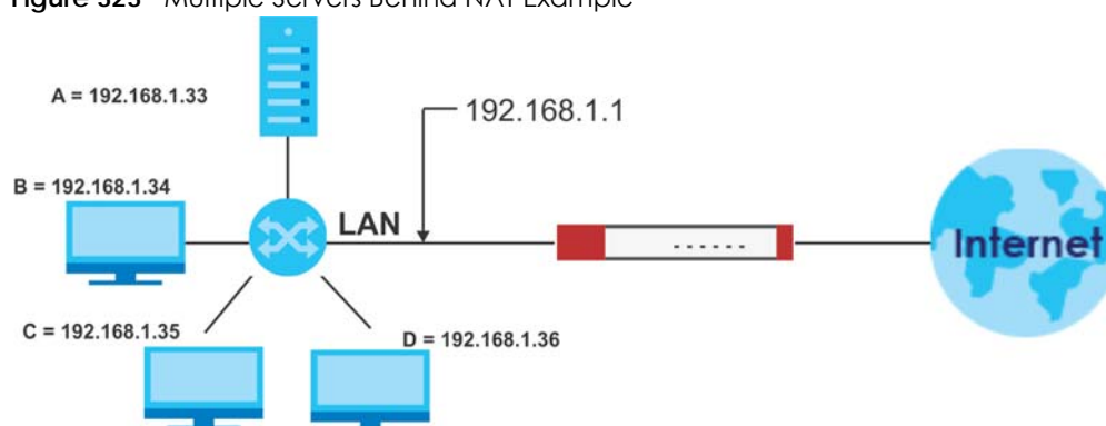
Figure 323 Multiple Servers Behind NAT Example
