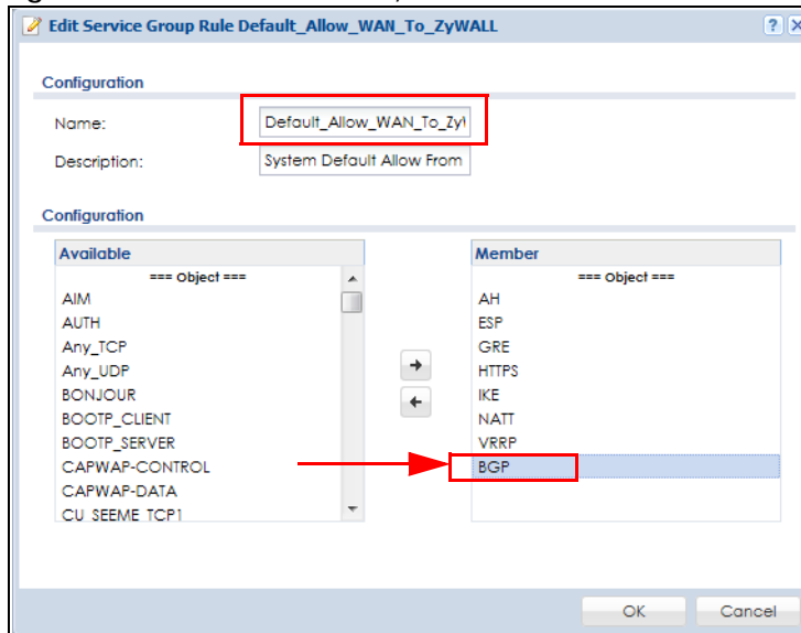
Figure 316 Allow BGP to the Zyxel Device
