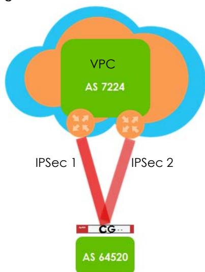
Figure 448 CG - to - Amazon VPC
