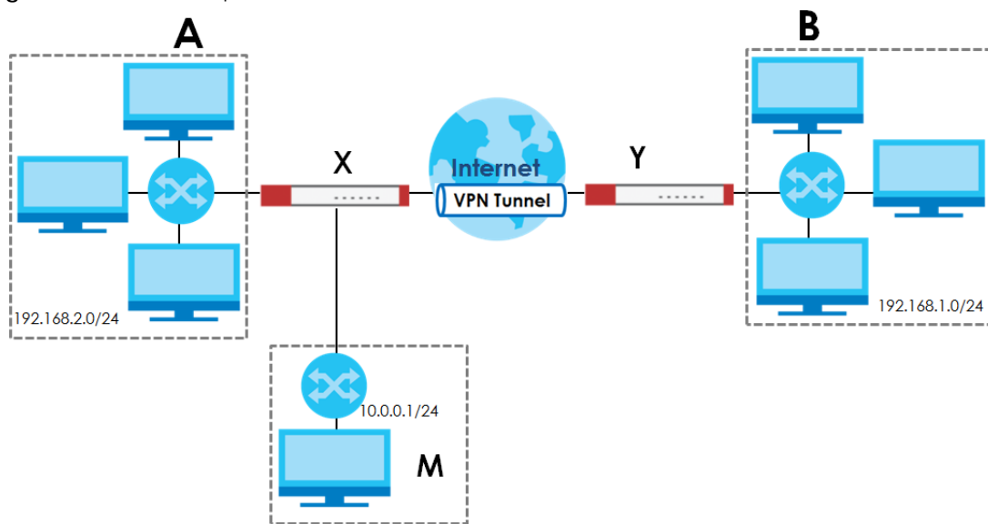
Figure 467 VPN Example: NAT for Inbound and Outbound Traffic
