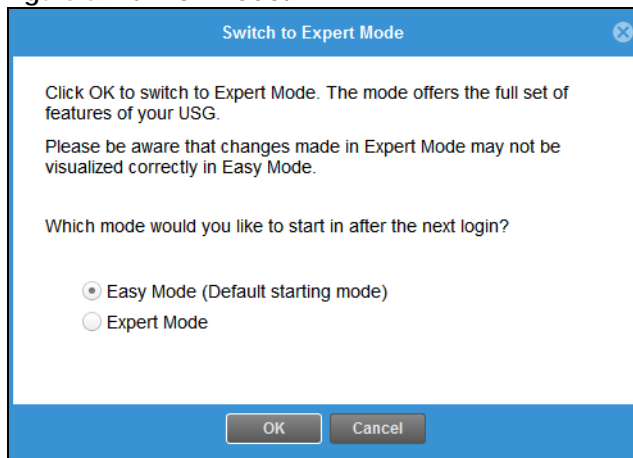
Figure 69 Switch Modes
