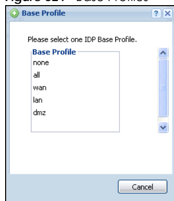
Figure 521 Base Profiles
