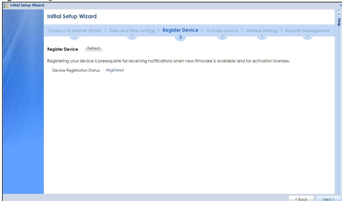
Figure 35 Registered Device
