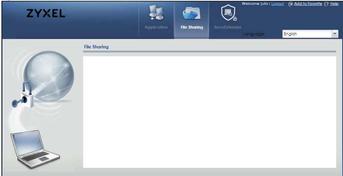
Figure 483 File Sharing
