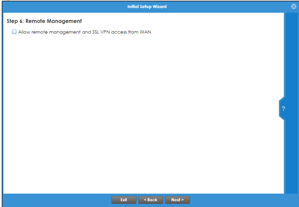
Figure 82 Remote Management
