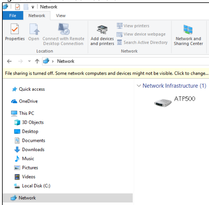
Figure 359 Network Connections
