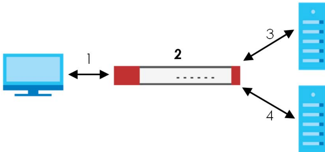
Figure 254 RTLS Example
