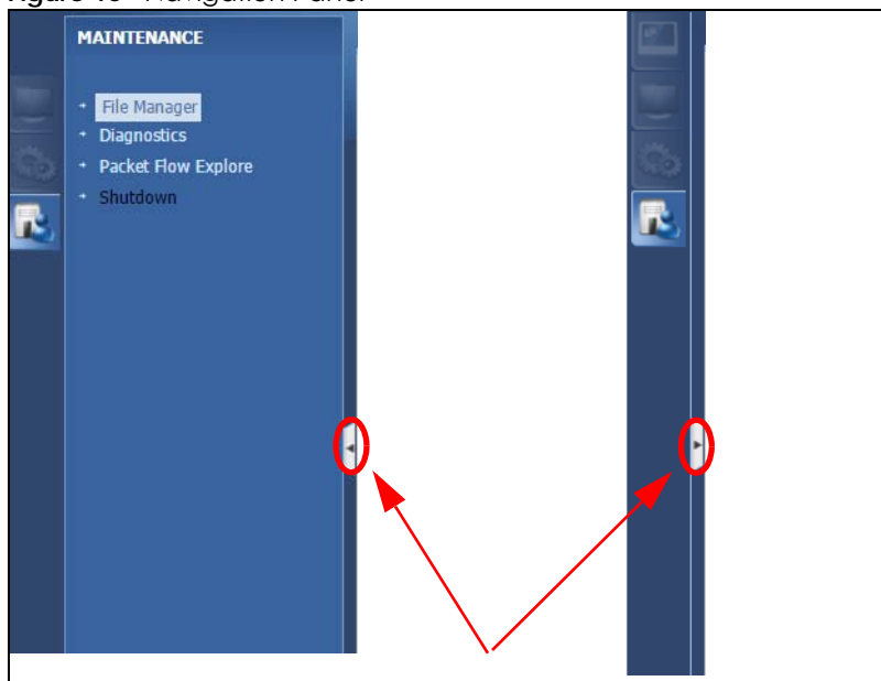
Figure 16 Navigation Panel
