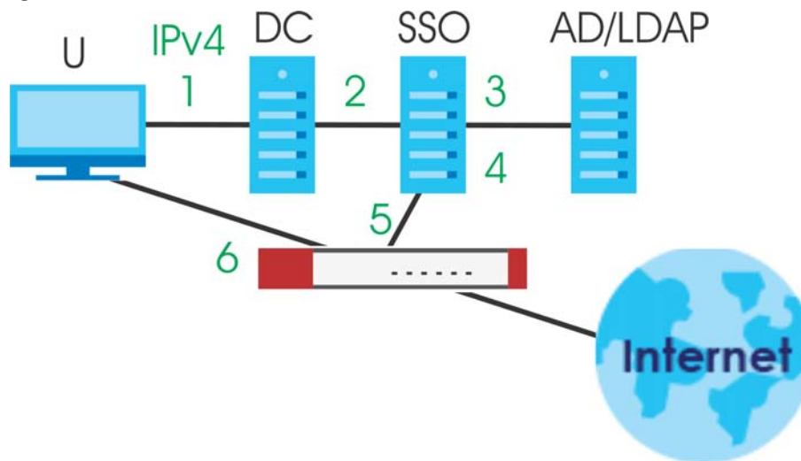
Figure 394 SSO Overview
