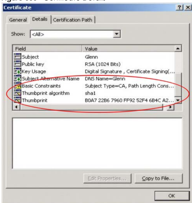
Figure 636 Certificate Details
