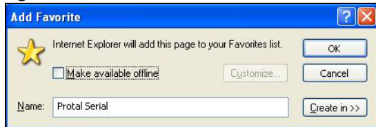
Figure 480 Add Favorite
