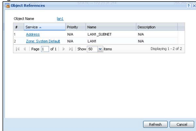
Figure 269 References
