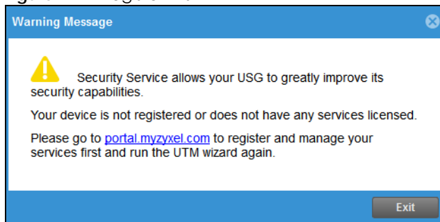
Figure 117 Register First
