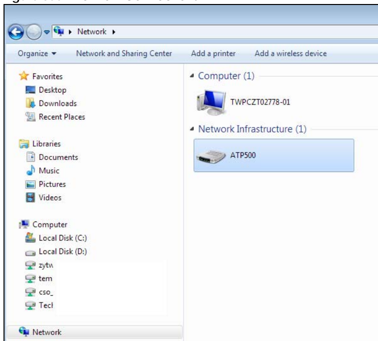
Figure 356 Network Connections
