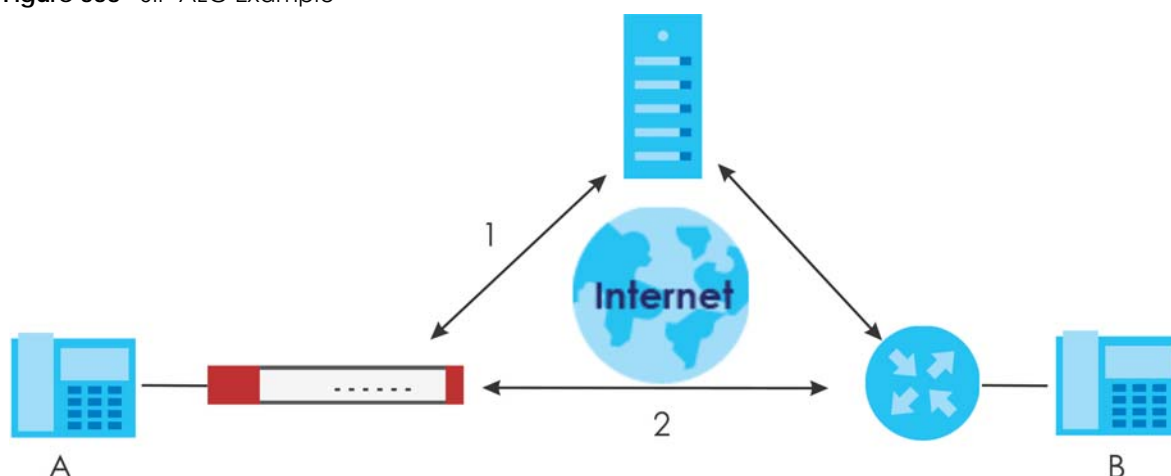
Figure 338 SIP ALG Example
