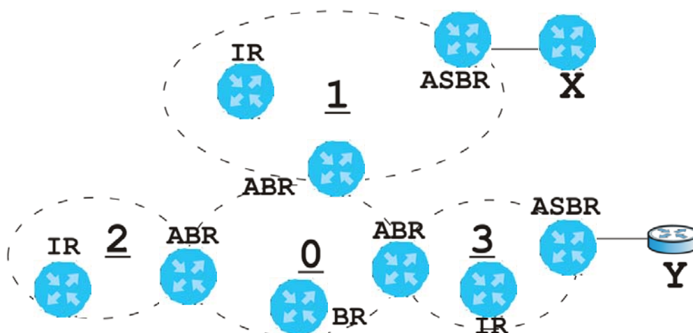
Figure 310 OSPF: Types of Routers
