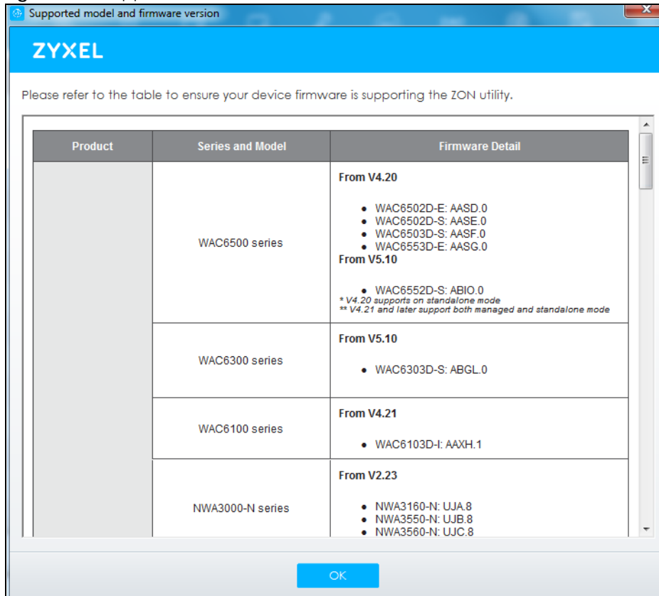
Figure 709 Supported Devices and Versions
