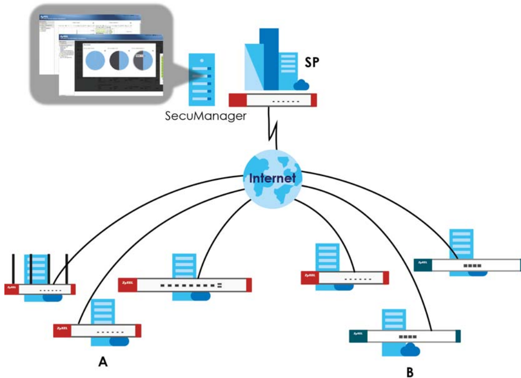
Figure 441 Cloud CNM SecuManager Example Network Topology
