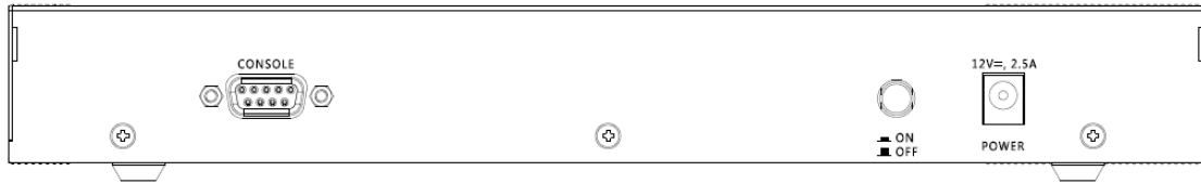
Figure 61 VPN100 Rear Panel
