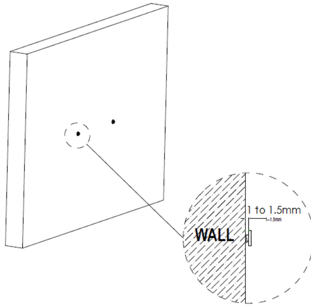
Figure 68 Gap for Cables
