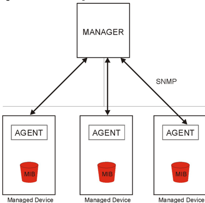
Figure 699 SNMP Management Model
