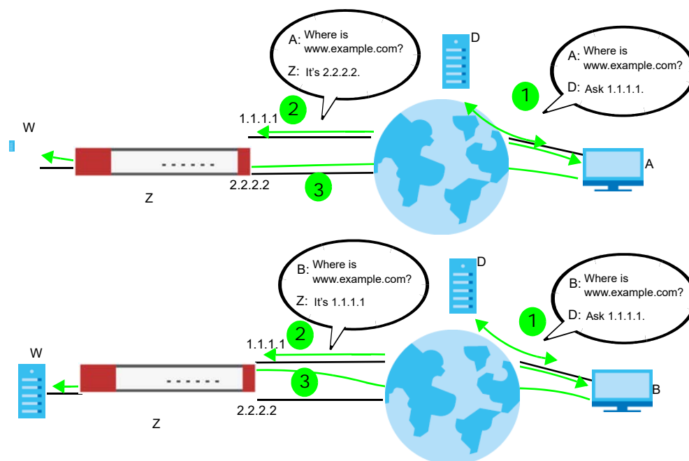
Figure 371 DNS Load Balancing Example
