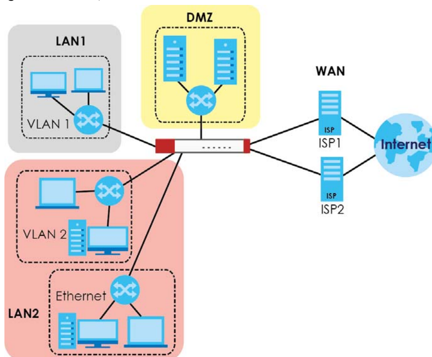
Figure 565 Example: Zones
