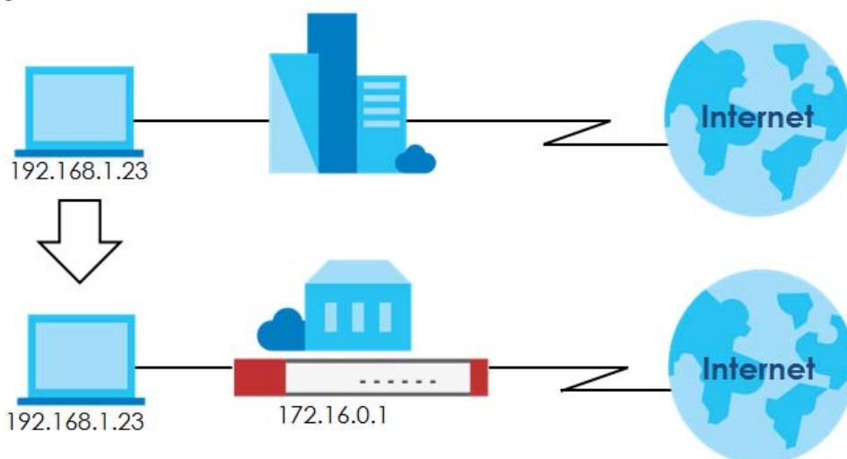
Figure 416 IPnP Application
