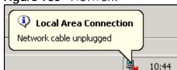
Figure 735 Network
