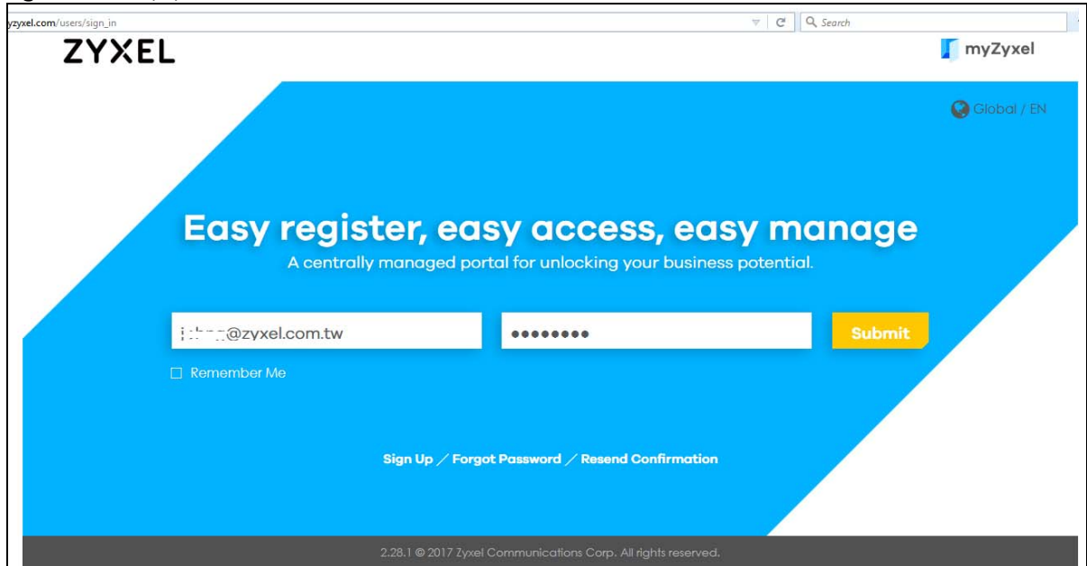
Figure 123 MyZyxel Portal
