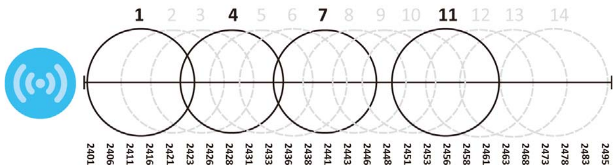
Figure 257 An Example Four-Channel Deployment
