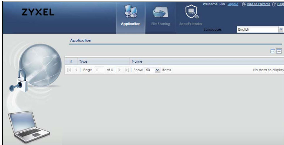
Figure 482 Application
