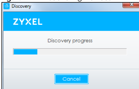
Figure 711 Discovering Devices
