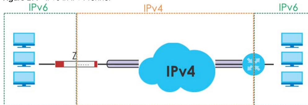
Figure 279 IPv6-in-IPv4 Tunnel
