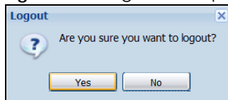
Figure 481 Logout: Prompt
