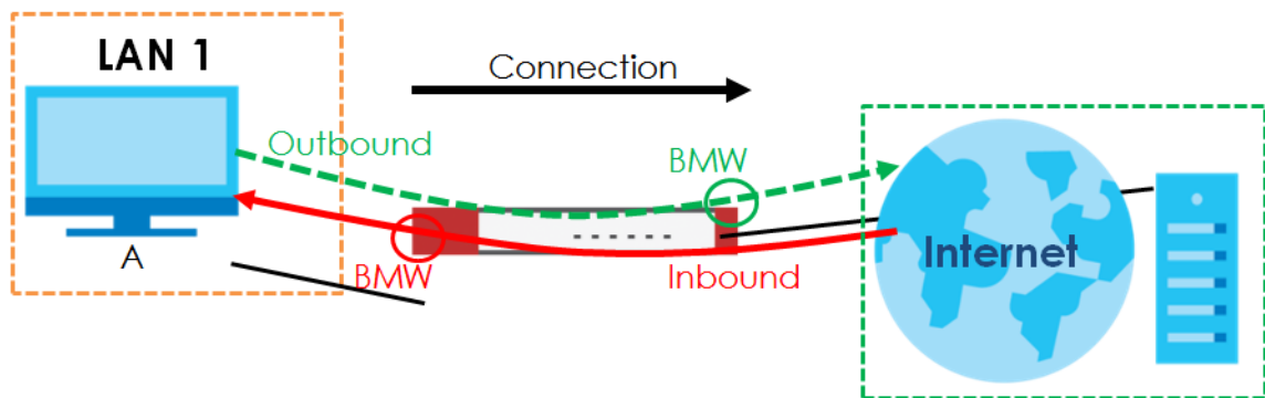
Figure 502 LAN1 to WAN Connection and Packet Directions
