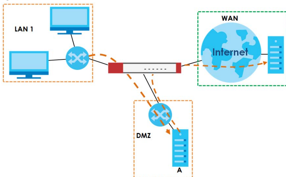
Figure 334 HTTP Redirect Example
