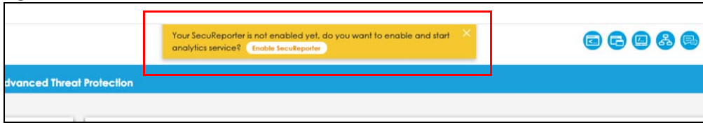
Figure 445 SecuReporter Banner
