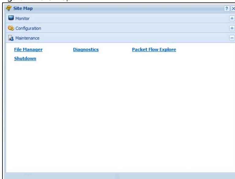
Figure 14 Site Map
