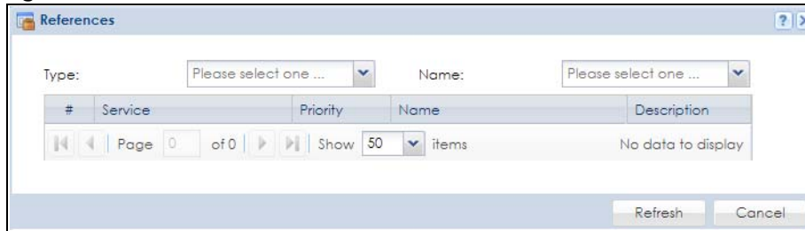
Figure 12 Reference
