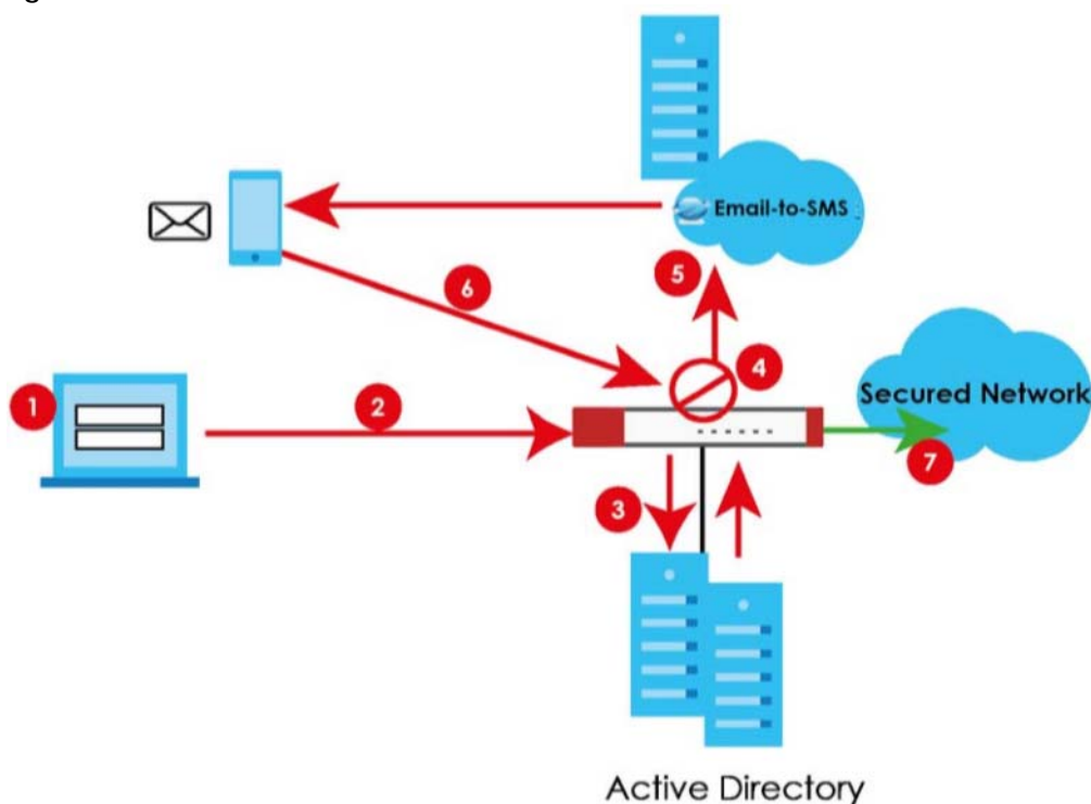
Figure 632 Two-Factor Authentication
