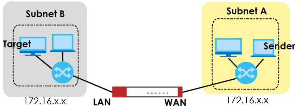
Figure 266 Proxy ARP
