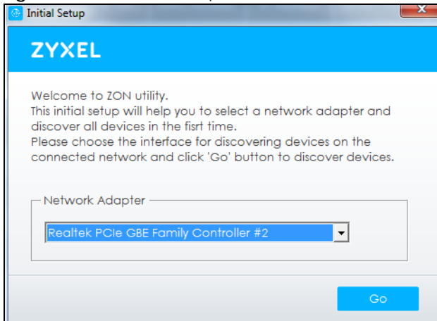
Figure 710 Network Adapter
