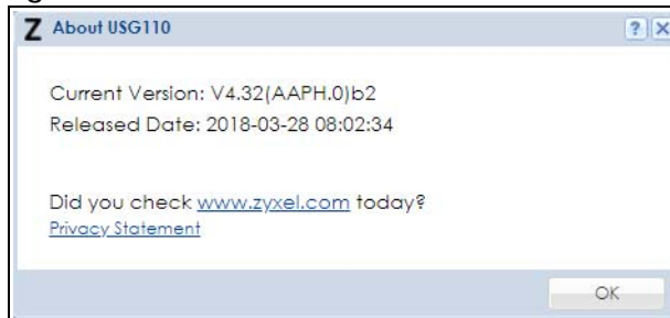
Figure 15 About
