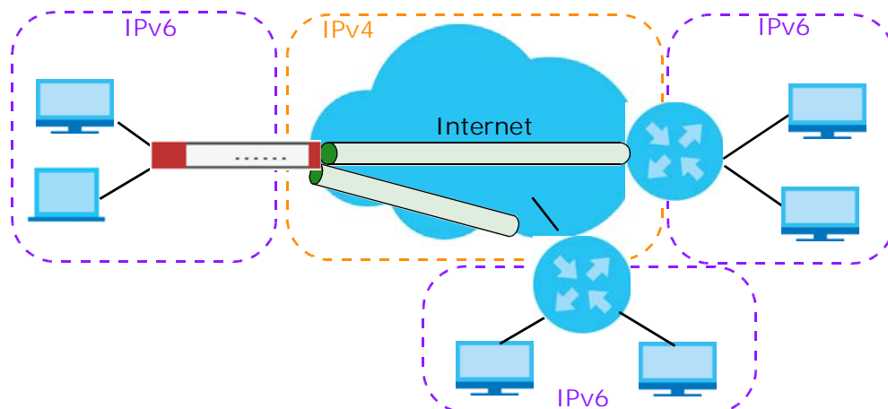
Figure 280 6to4 Tunnel
