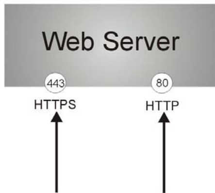
Figure 669 HTTP/HTTPS Implementation
