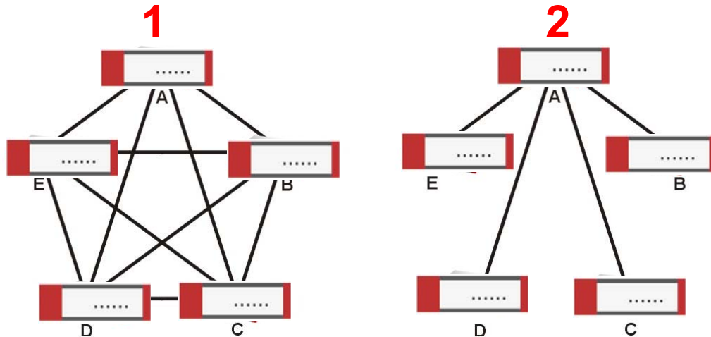
Figure 458 VPN Topologies (Fully Meshed and Hub and Spoke)
